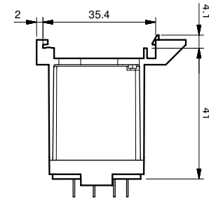
055.17 with relay
