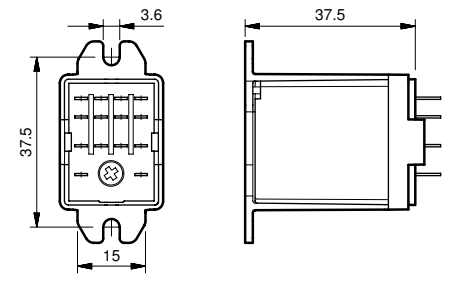
055.15 with relay
